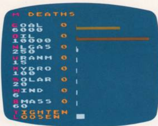
Figure 7. DEATHS Graph for 1980, PRO FOSSIL Bias
