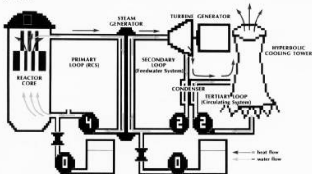
Figure 1. Heat Transfer in the PWR System
