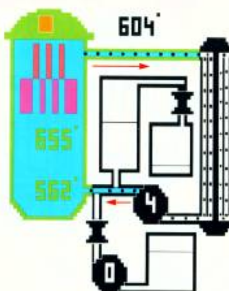
Figure 4. The Reactor Vessel
