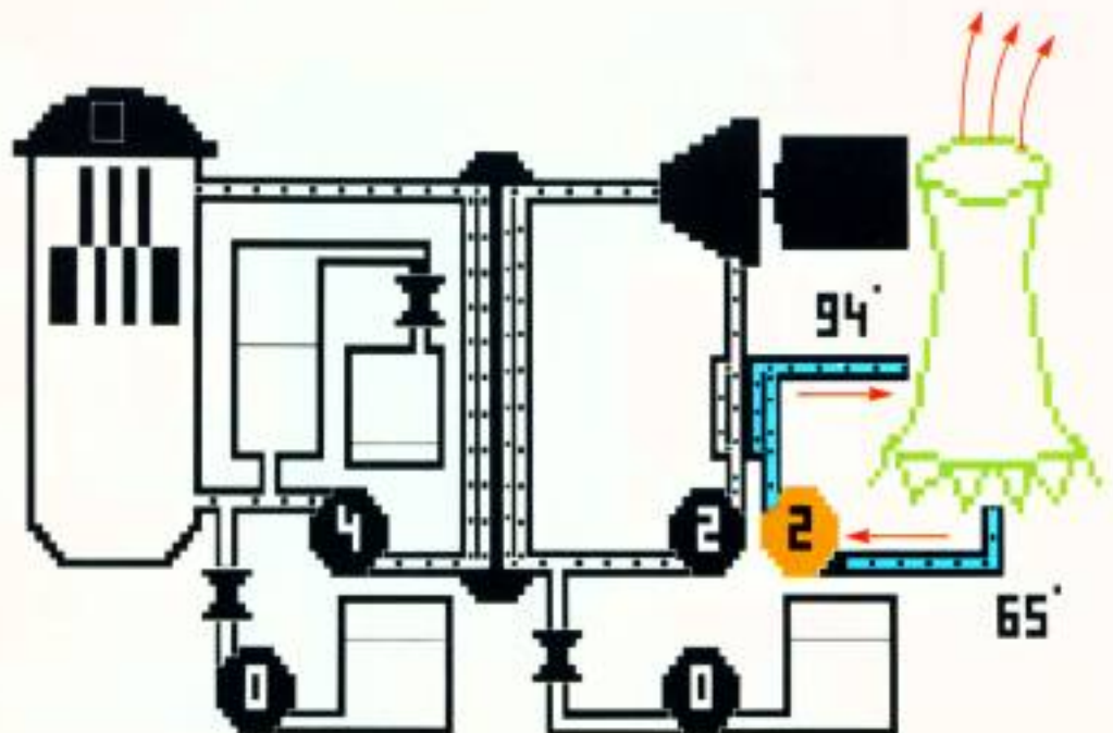
Figure 9. Cooling Tower
