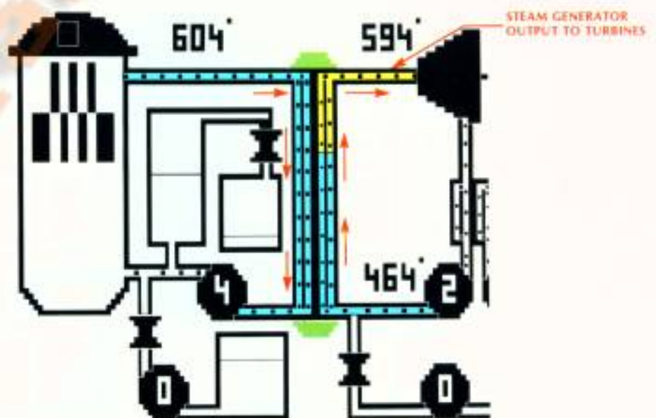
Figure 6. Steam Generator
