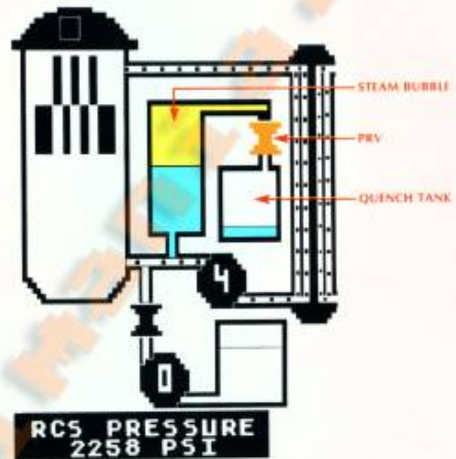
Figure 5. The Pressurizer
