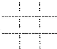
Figure 1 Game Grid
