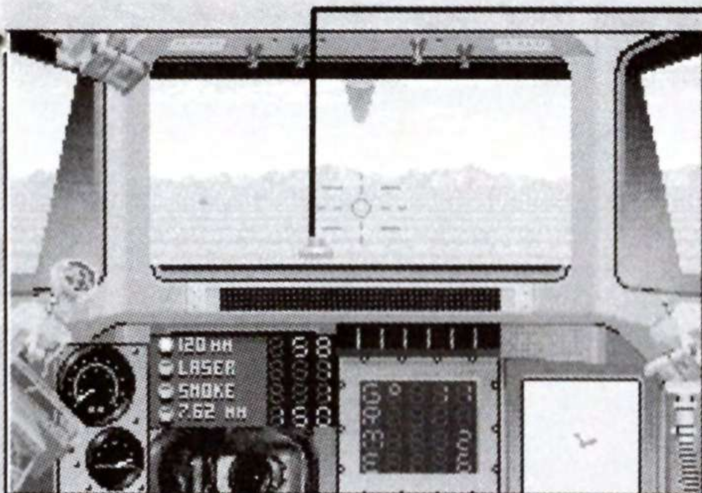
Minefield Screen
